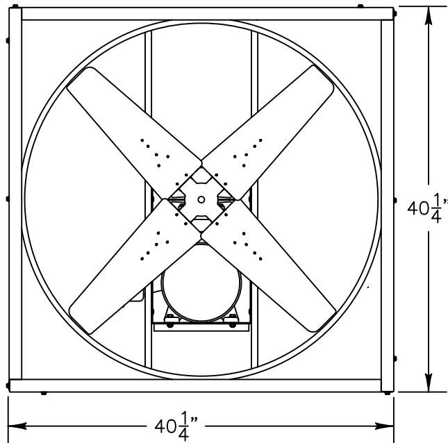
DISCHARGE VIEW
