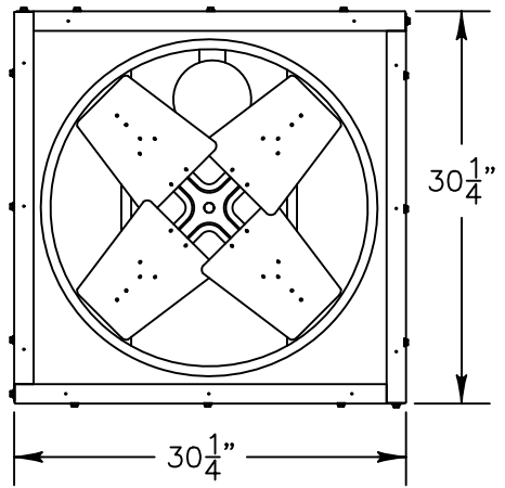
DISCHARGE VIEW
