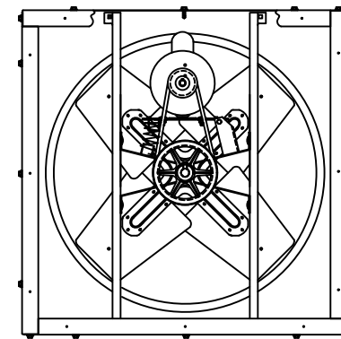
INTAKE VIEW
