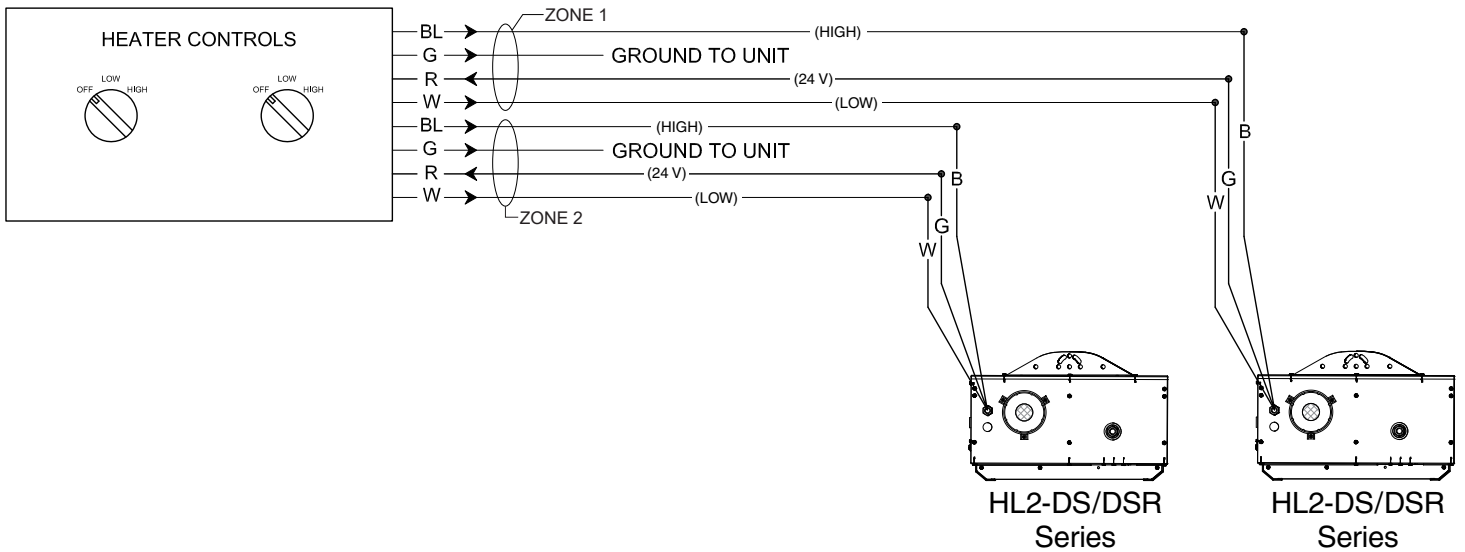
Figure 4 • Two Stage Wiring for Multiple Heaters (TH-DSTS2)
