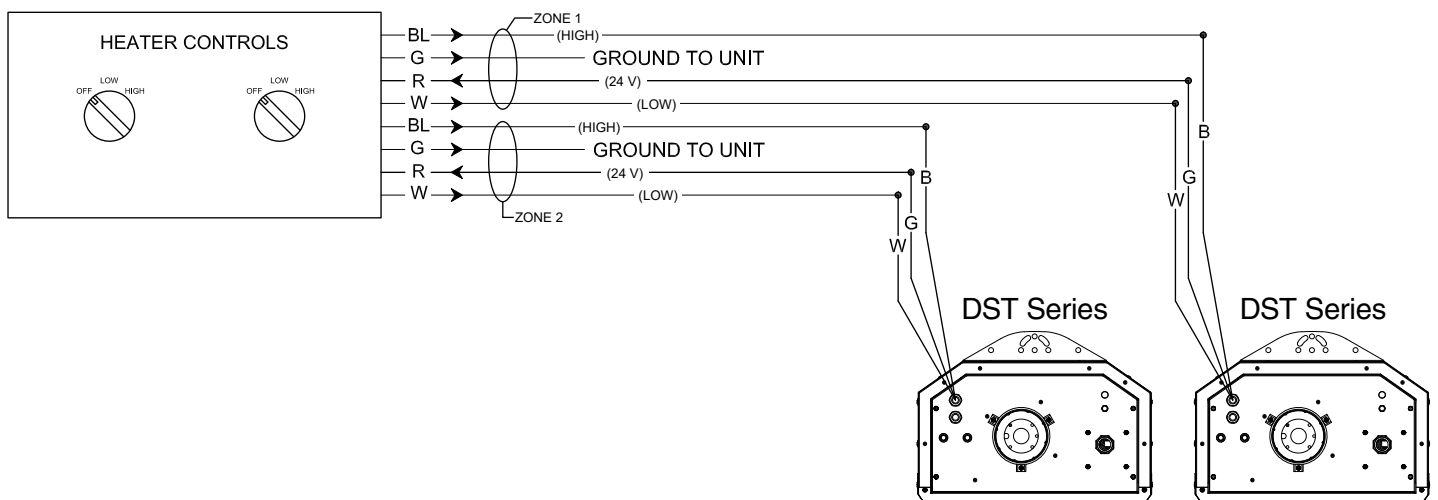
Figure 2 • Two Stage Wiring for Multiple Heaters (TH-DSTS2)
