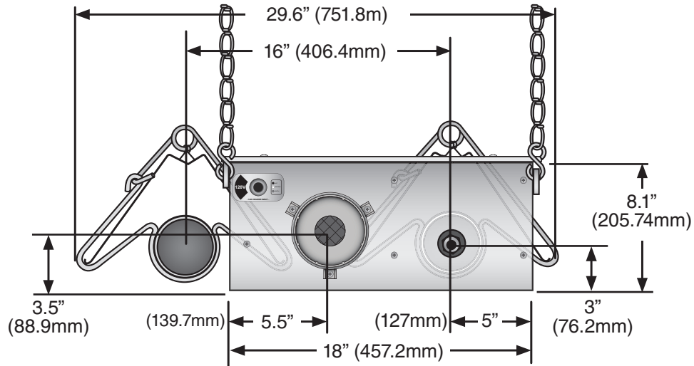
Figure 4 • Burner Control Box Dimensions - End View
