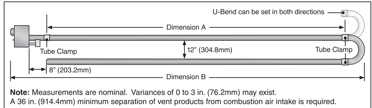
Figure 1 • Dimensions for Heater Installed with U-tube Fitting (P/N: TF1B)
