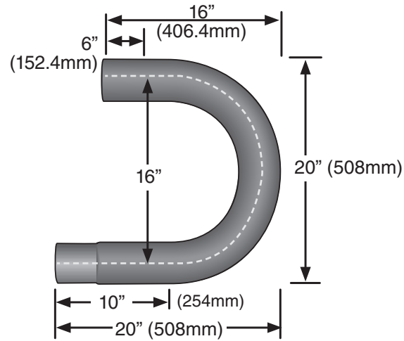
Figure 3 • TF1B U-tube Dimensions
