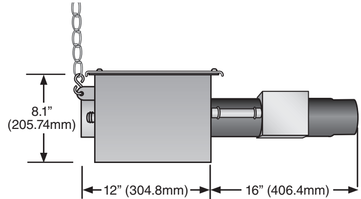
Figure 5 • Burner Control Box Dimensions - Side View
