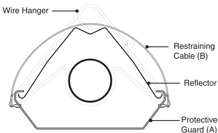
Figure 2 • Protective Guard • End View
