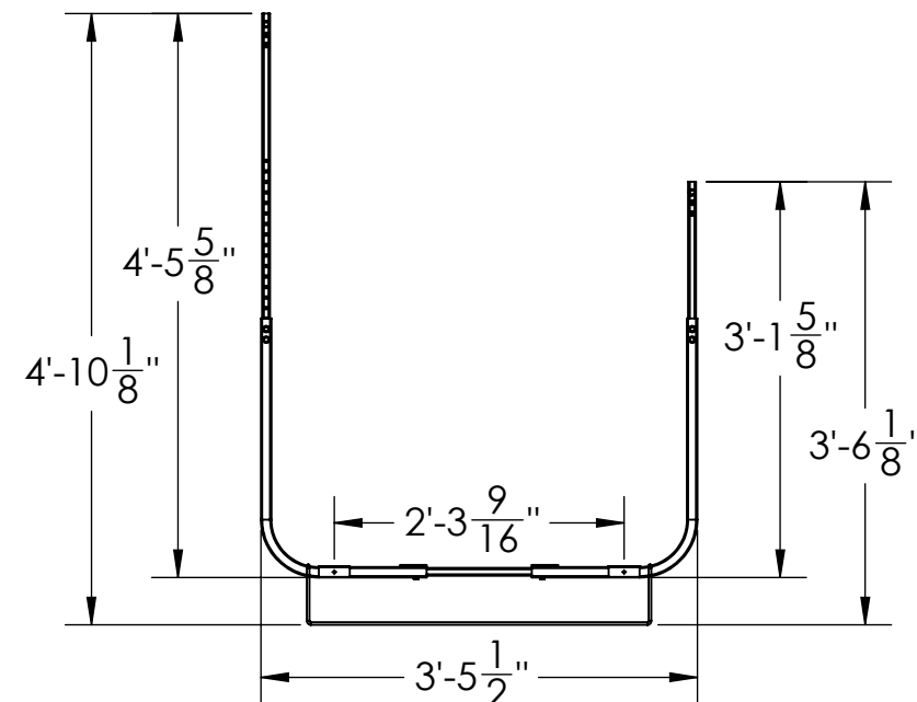
END VIEW RETRACTED
