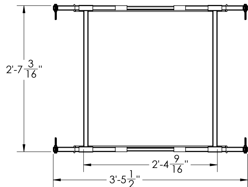
PLAN VIEW RETRACTED
