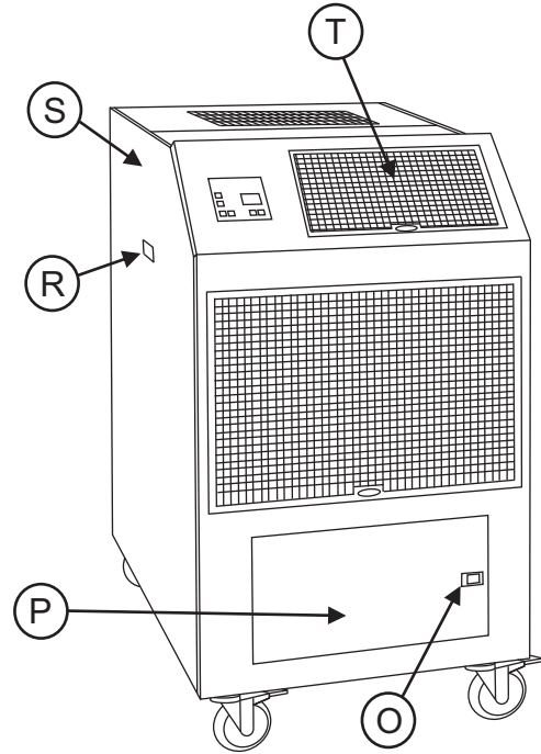
FRONT/LEFT SIDE
