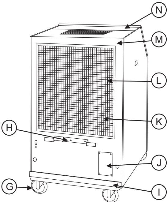
REAR/LEFT SIDE
