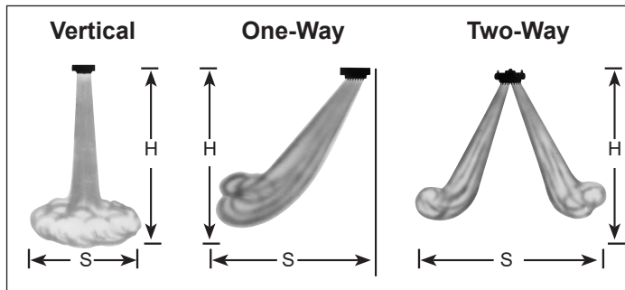
Figure 7.7 - With One- or Two-Way Louvers
