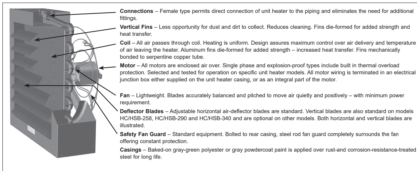
Figure 4.1 - Unit Features
