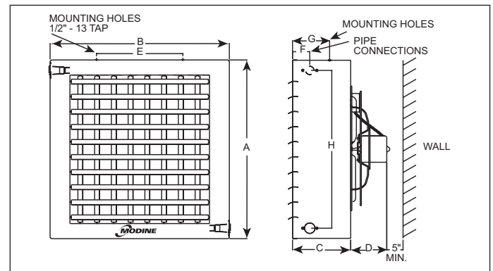
Figure 25.4 - Model Dimensions HC 193-340 ①
