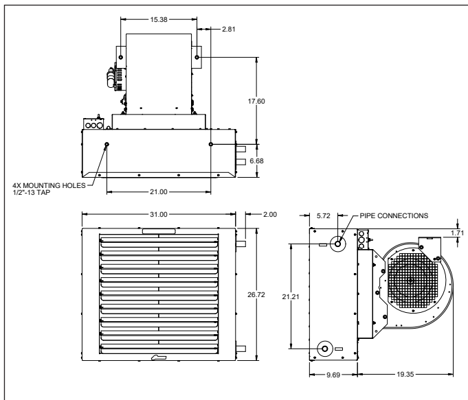
Figure 26.2 - Model Dimensions BCH 103
