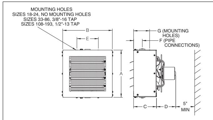
Figure 25.3 - Model Dimensions HC 18-165
