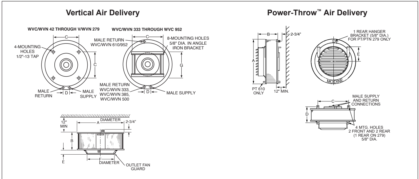
Figure 27.1 - Model V/VN and PT/PTN Dimensions
