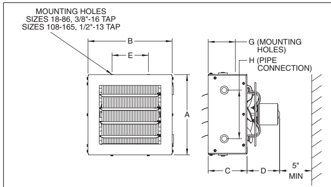
Figure 26.1 - Model Dimensions HCH 22-195
