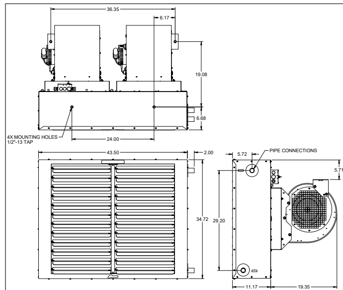
Figure 26.3 - Model Dimensions BCH 218
