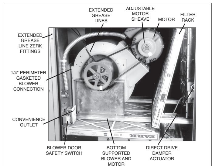
Figure 26.4 Blower Section
