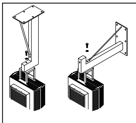
WALL / CEILING BRACKET
