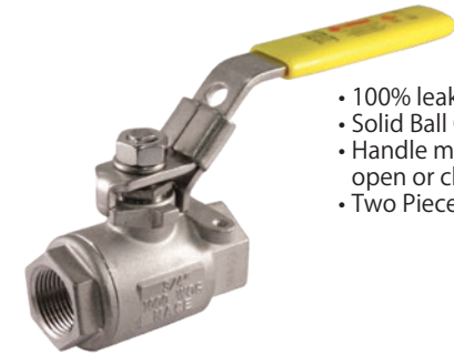
T-SS-2000N-DH 2 Piece • Full Port • Threaded Connection • 2000 WOG • with Spring Return Handle
