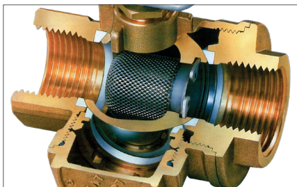
3-Way Ball Valve
