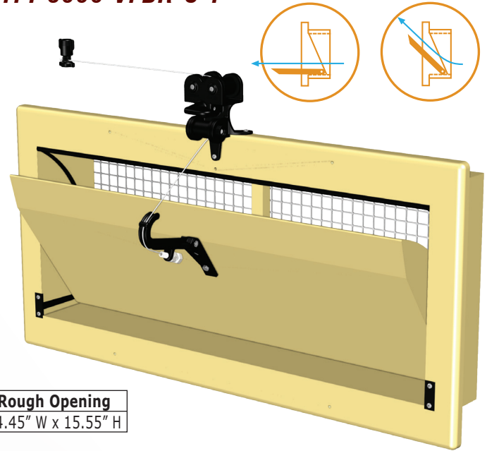
TPI-3000-VFBR-C-Y Air Inlet
