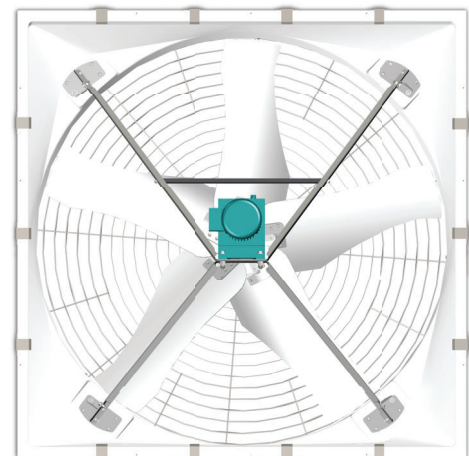
Shown with shutter removed. Never provide power to fan without guards and shutter properly installed.
