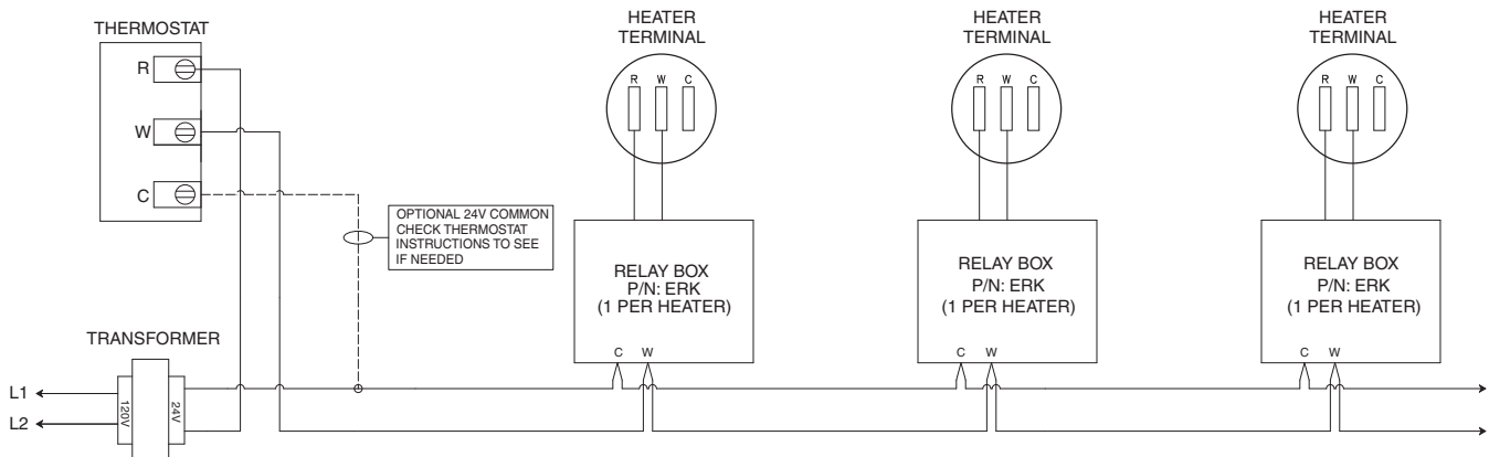
Figure 2.3 • Multiple Heaters, Single Thermostat Connection with External Relay Kit
