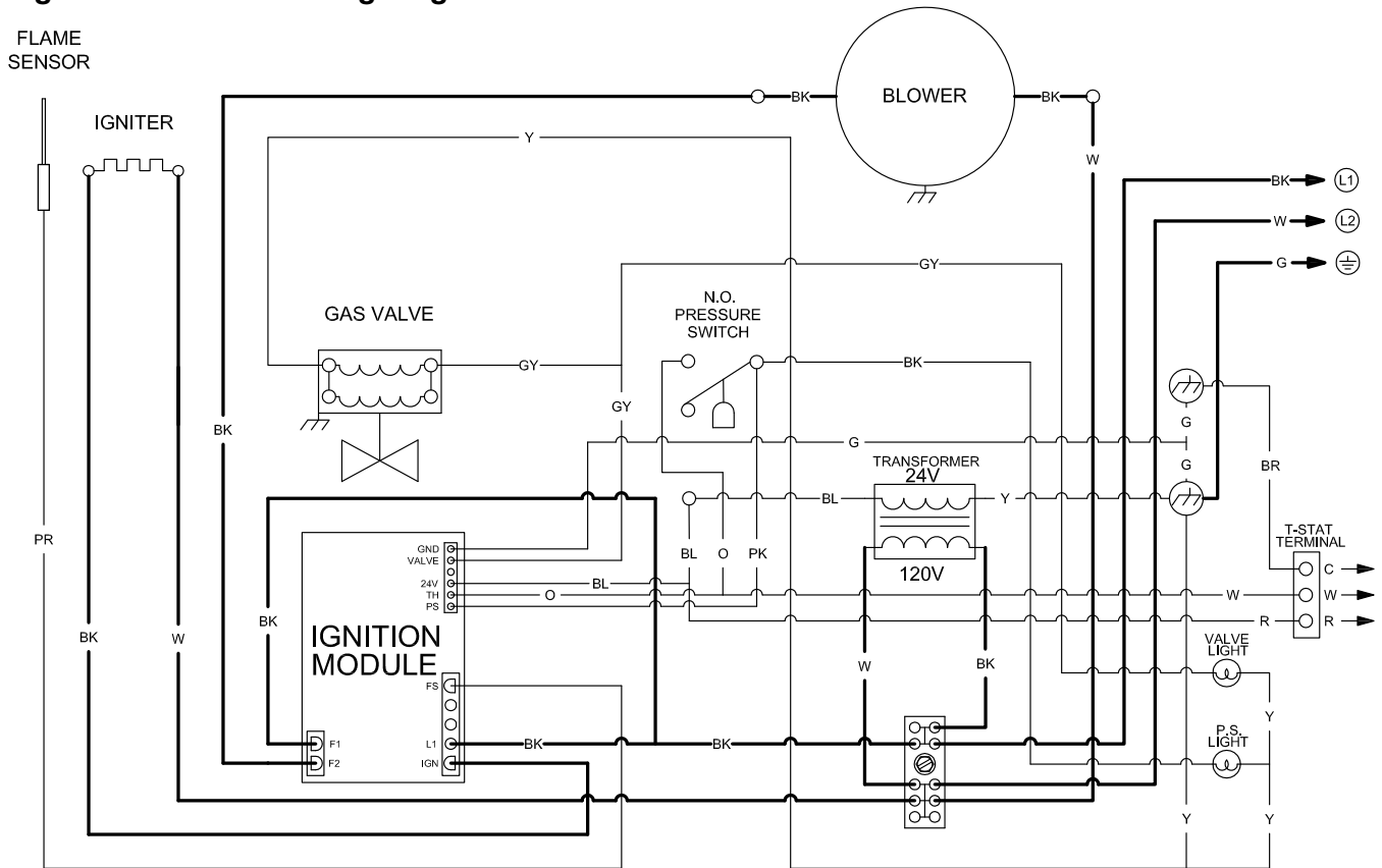
Figure 2.1 • Internal Wiring Diagrams
