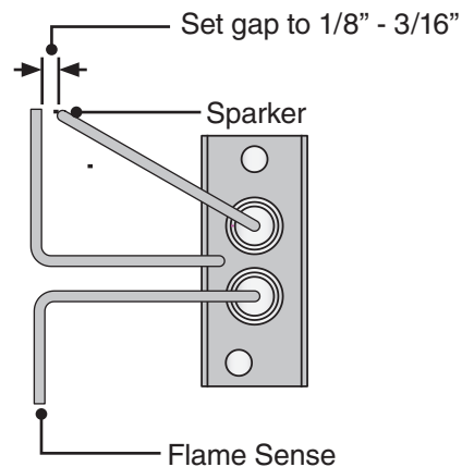
Figure 3 • Replacement 32-508 Electrode Top View
