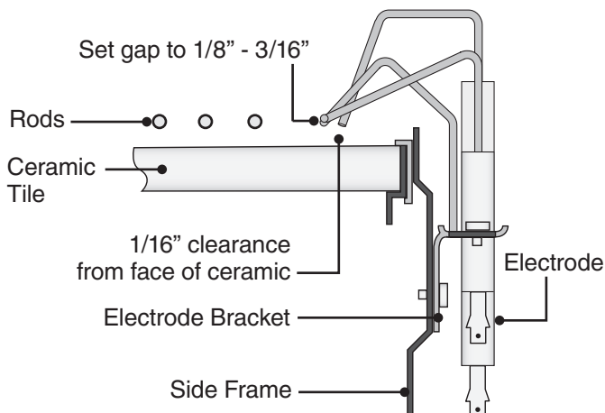
Figure 2 • Replacement 32-508 Electrode Side View
