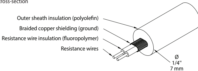
Figure 1: Cable cross-section
