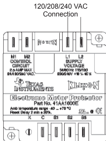
Figure 2 41AA Wiring Connections for Module
