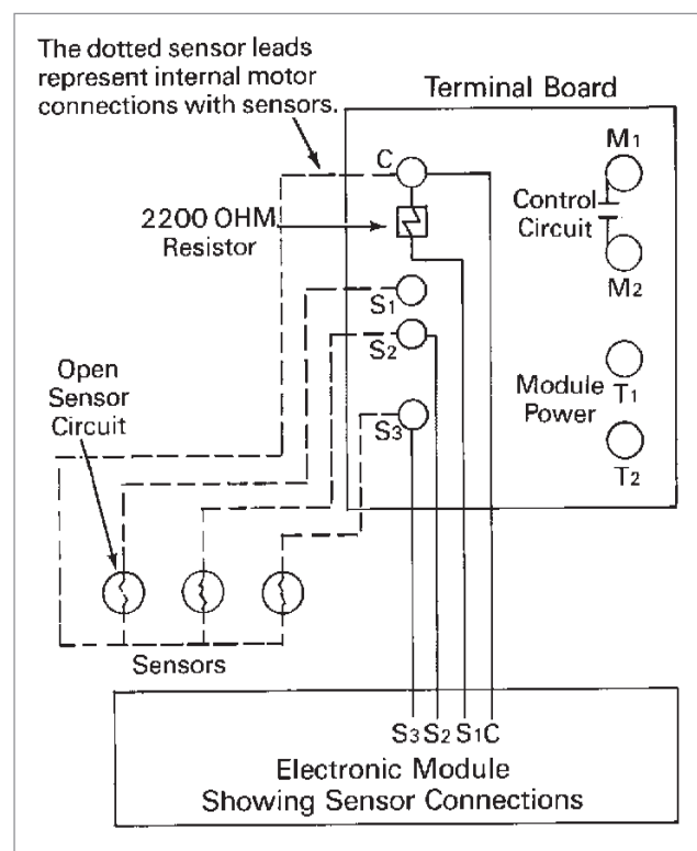
Figure 9 Emergency Bypass of Damaged Solid State Sensor
