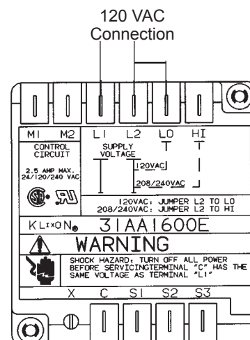
Figure 4 31AA Wiring Connections
