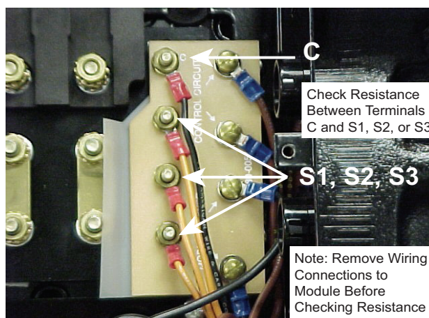
Figure 8 Checking Resistance Through Solid State Sensors
