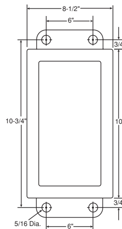
STAR-GF Mounting Dimensions
