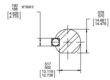
SECTION B-B SHAFT DETAIL
