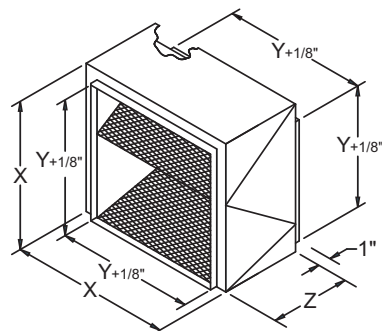
FILTER SECTION
