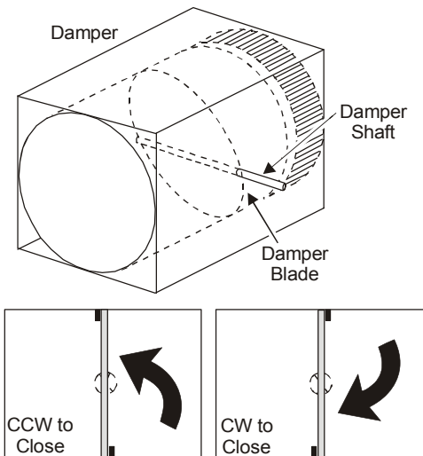
Figure 3: Damper Rotation
