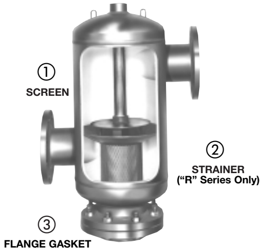
“R” SERIES WITH STRAINER
