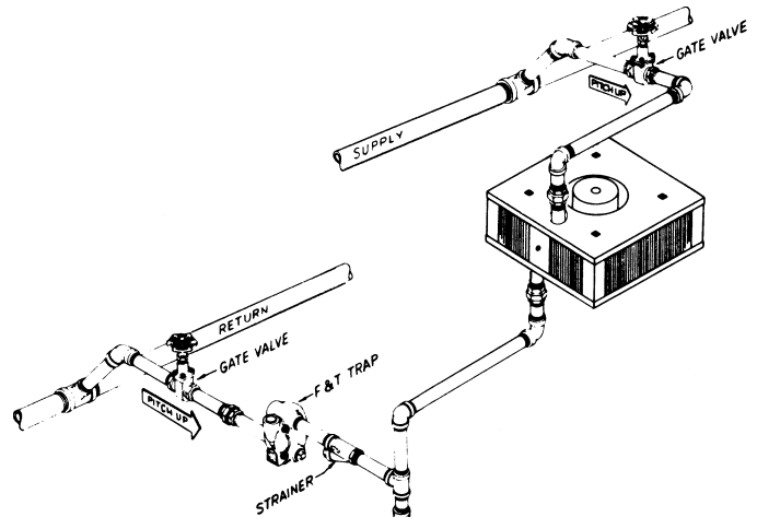
Figure 9 – Low Pressure Vapor or Vacuum
