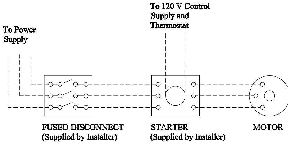
Figure 13 - Fan Motor Connections 3 Phase Wiring
