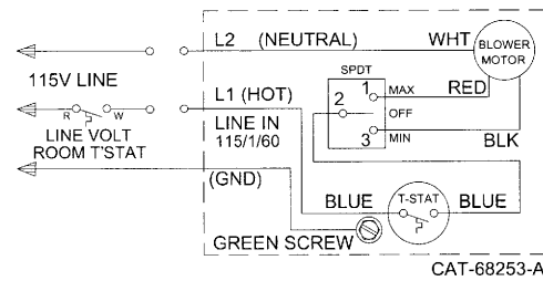
WIRING DIAGRAM 2
