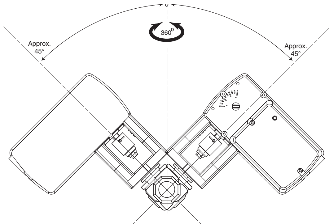
Figure-12 Acceptable Mounting Orientation for Steam Applications
