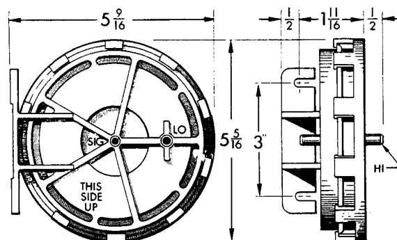
Figure-2 Dimensions.
