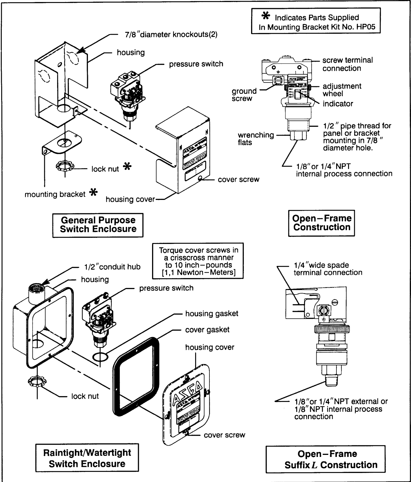
Figure 3. H-Series pressure switches.
