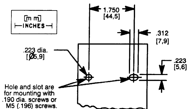
Figure 2. General purpose enclosure.
