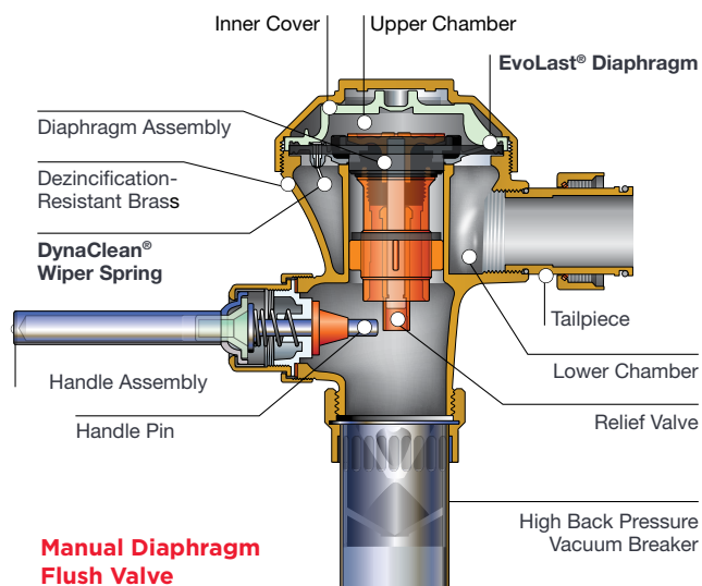
Selectronic Diaphragm Flush Valve
