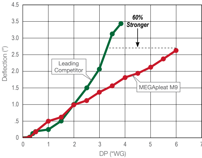
Results from a wet breach test performed at an independent test lab shows the MEGApLeat® M9 filter is over 60% stronger than the leading competitor.
