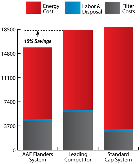
Analysis based on a 3-stage filter system, running 20,000 CFM, over a 2 year time period. Energy costs based on the national average of 0.08 $/kW-hr. Filter selection was based on the most energy efficient filters available.
